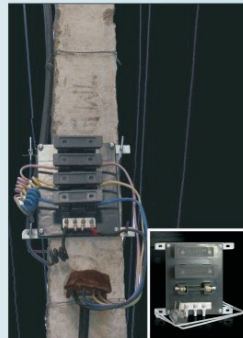
60A Fuse Board
